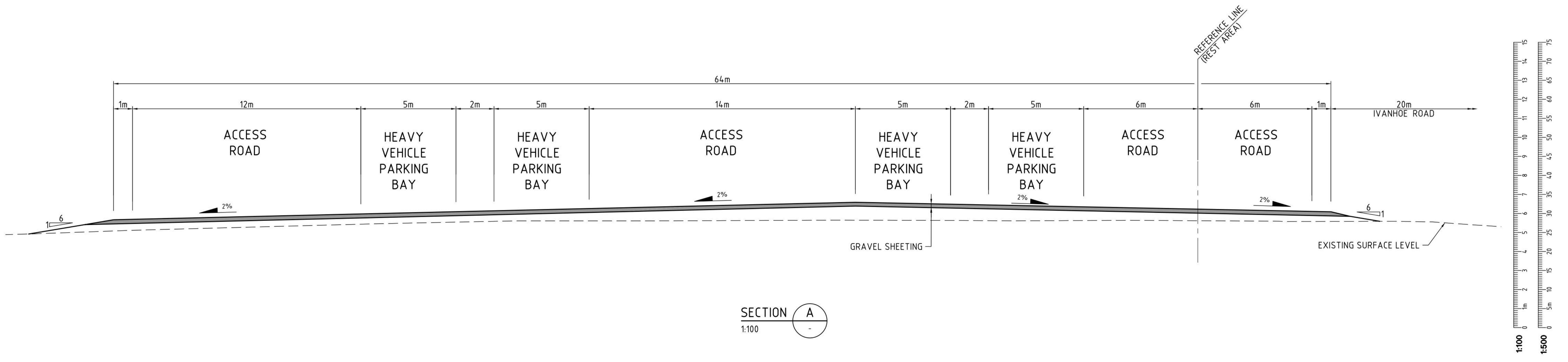
IVANHOE ROAD REST AREA SCALE: 1:500
