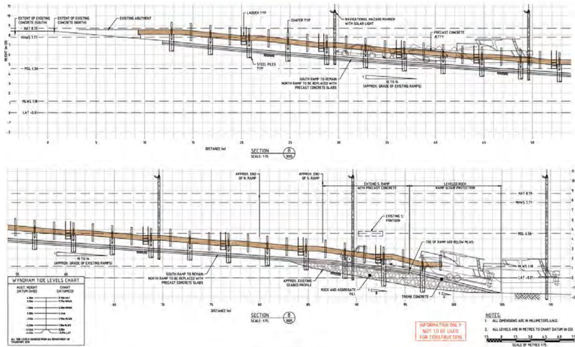
Figure 6-10 Typical Section – Fixed Jetty Option
